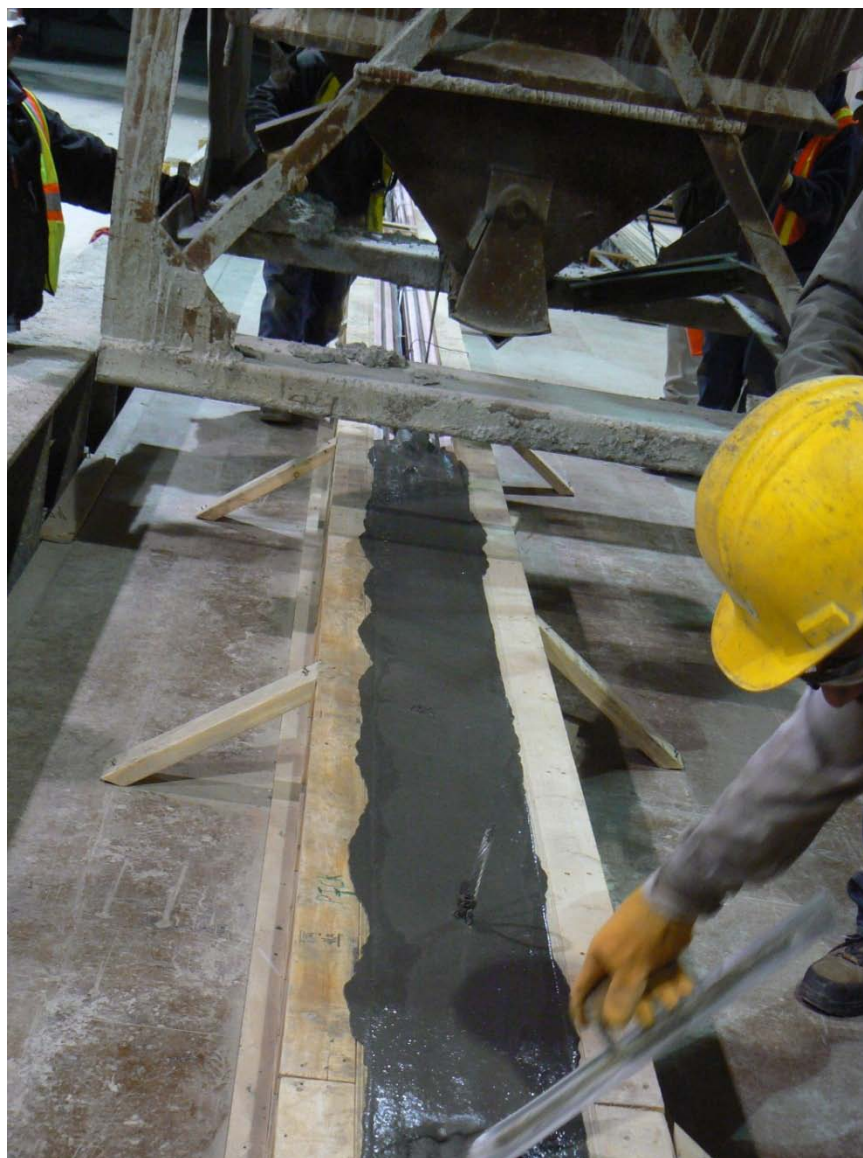
Figure 4.19. Pouring of 35-ft (10.7-m) long UHPC pile P1
