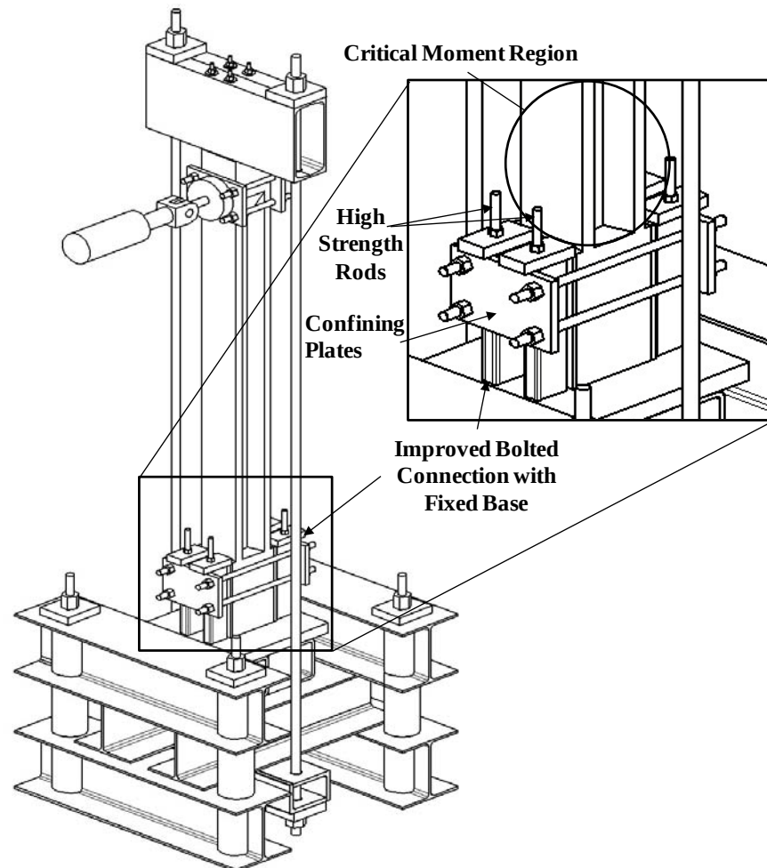
Figure 4.31. Laboratory test setup with bolted connection at the base for UHPC test unit L2
