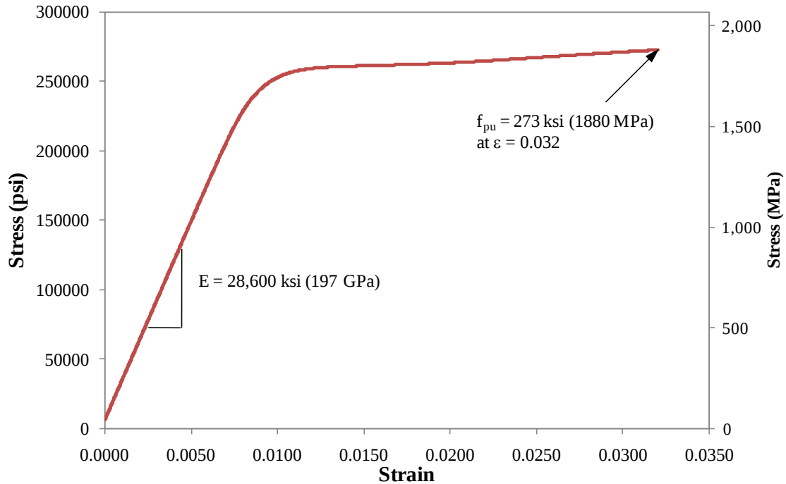
Figure 4.27. Measured stress-strain behavior of a ½-in. (13-mm) diameter low relaxation prestressing strand
