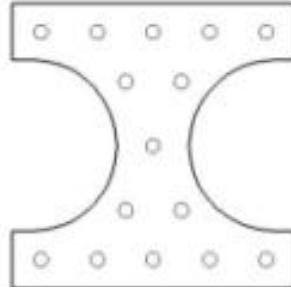
Figure 3.5. X-shaped section considered for UHPC pile
