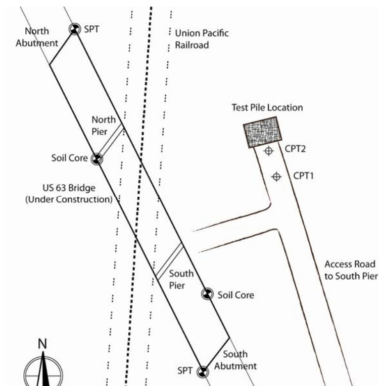
Figure 5.1. Plan view of the Oskaloosa bridge site including locations of test piles
