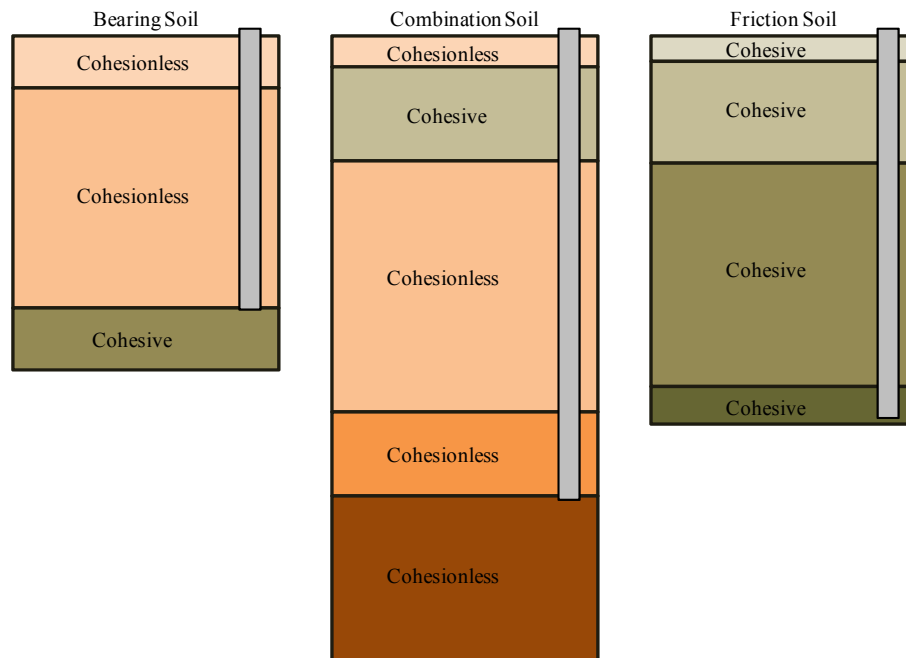
Figure 3.16. Soil profiles used in driveability analysis
