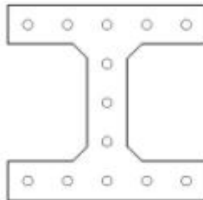
Figure 3.4. Simple H-shaped section considered for UHPC piles
