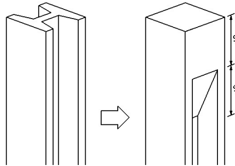
Figure 3.15. Expanded region at top of UHPC piles to minimize driving stresses
