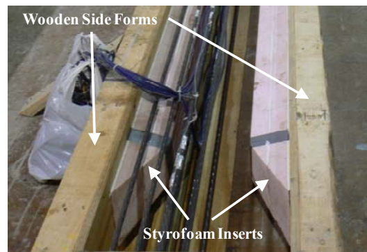
Figure 4.9. Formwork used for casting of tapered H-shaped section
