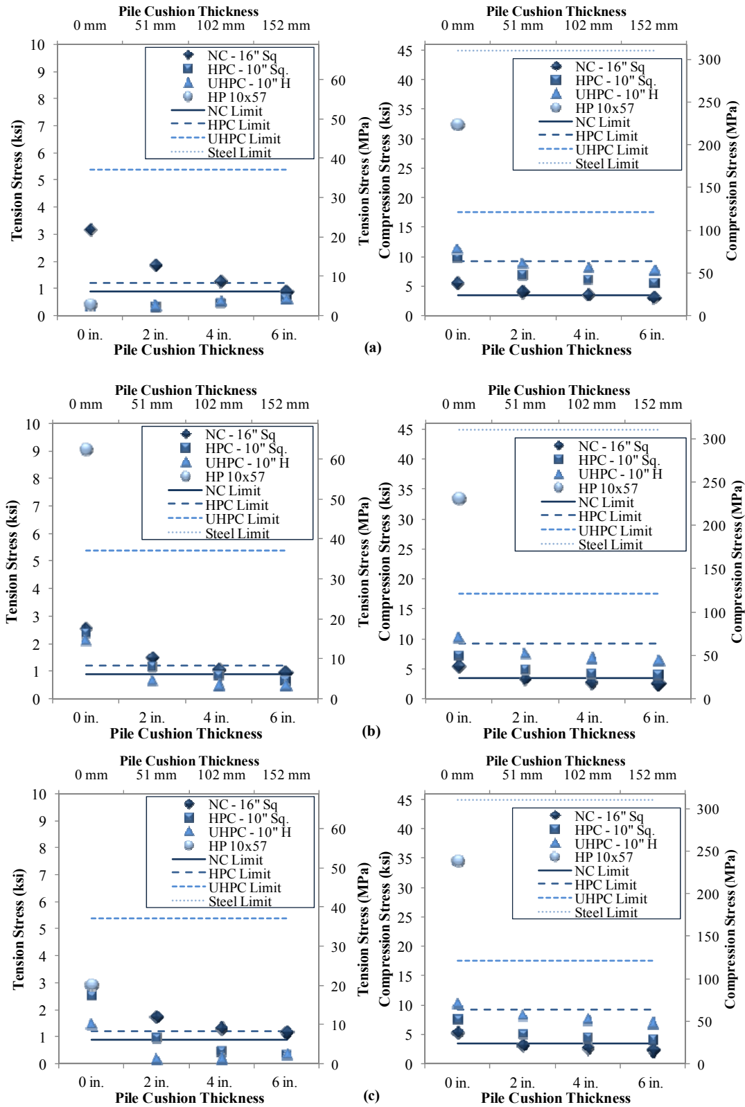
Figure 3.17. Tension and compression stresses with a D19-42 hammer and 10-ft (3.0-m) stroke in (a) Bearing Soil, (b) Combination Soil, and (c) Friction Soil
