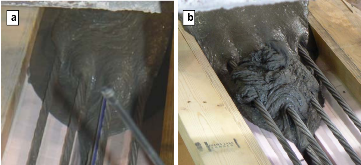
Figure 4.23. Comparison of flowability of a) first and b) second pour of UHPC
