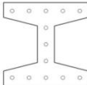
Figure 3.6. Tapered H-shaped section considered for UHPC pile
