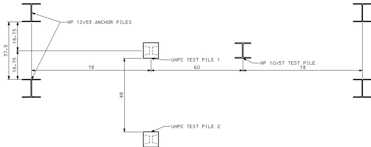
Figure 5.14. Configuration of the test and anchor piles
