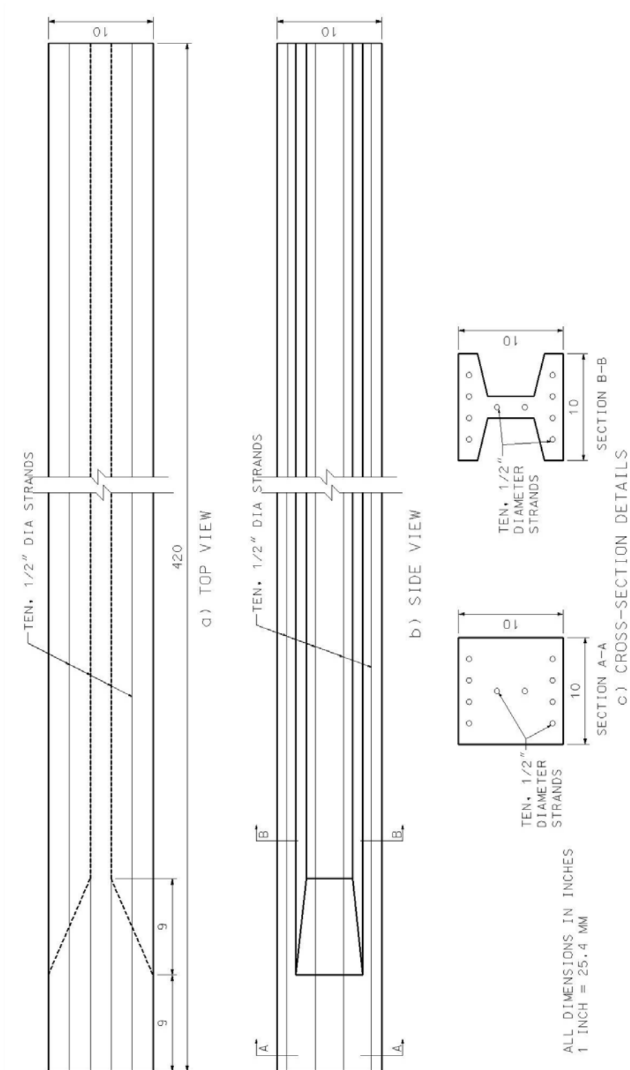
Figure 4.4. Dimensions and reinforcement details of the 35-ft (10.7-m) long UHPC piles for field tests
