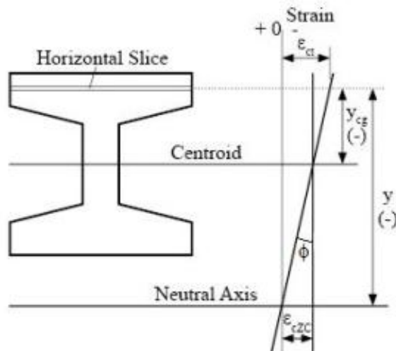
Figure 3.9. Definitions of distance from centroid and distance from neutral axis
