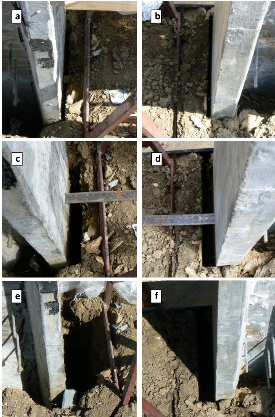
Figure 5.35. Soil gaps due to lateral pile movement next to a) P1 and b) P2 early in the test, c) P1 and d) P2 midway through the test, and e) P1 and f) P2 after shear failure of pile P1
