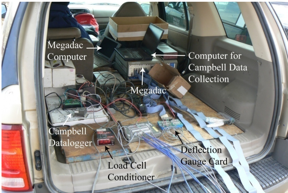
Figure 5.32. Data collection system used during the lateral load test
